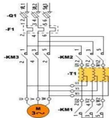
Auto-transformer starter
